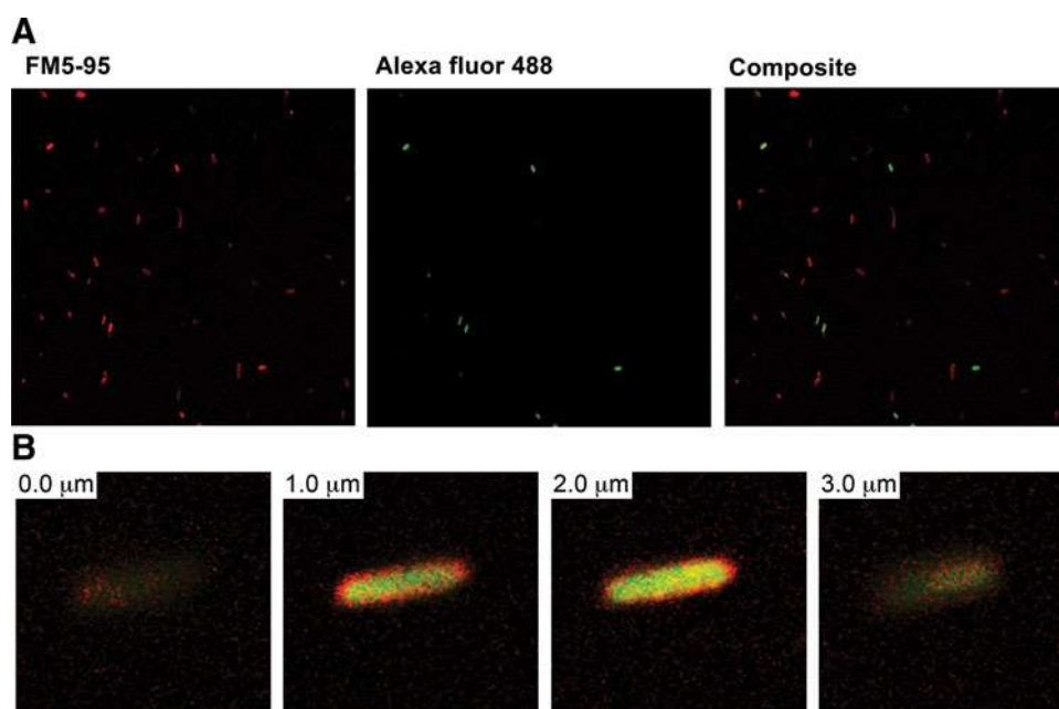
FIG. 3. Internalization of fLNA/DNA. (A) Cells in the stationary phase were incubated with fLNA/DNA as described in Materials and Methods, washed with phosphate-buffered saline, stained with FM5-95, and analyzed by laser scanning confocal microscopy. (B) Z-stack from a typical cell with internalized fLNA/DNA.
