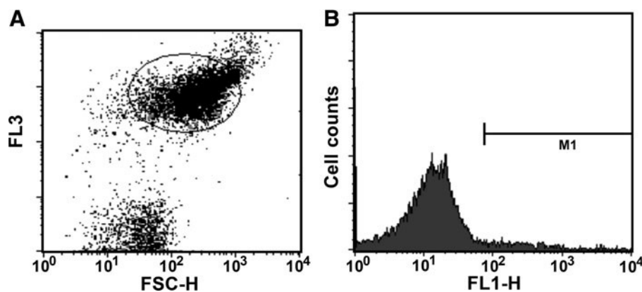
FIG. 1. Flow cytometry of fLNA/DNA cellular uptake. (A) Dot plot representing FSC-H (forward scattered) versus FL3. The inner circle represents the cells analyzed. (B) Histogram showing cell counters versus fluorescence from fLNA/DNA (FL1-H). M1 area represents percentage of cells containing Alexa Fluor 488.
