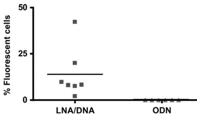
FIG. 2. Association of Escherichia coli cells with fLNA/DNA or fODN. The percentage of cells associated with fluorescence is compared for the fLNA/DNA (■) and fODN (▲). The averages, shown by horizontal lines were fLNA/DNA, 13.96 \pm 5.12, fODN, 0.05 \pm 0.01. The p value is 0.0349, p < 0.05 is considered significant.
