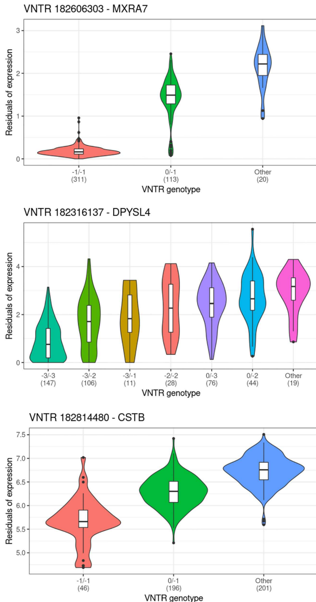
Figure 2. Gene expression differences and VNTR genotype. Shown are violin plots of gene expression values (log 2 normalized TPM) for three genes which displayed significant differential expression when samples were partitioned by VNTR allele genotype. Additional examples are shown in Supplementary Figures S26–S30. Genotype is indicated in labels on the X-axis and numbers refer to copies gained or lost relative to the reference allele. ‘Other’ indicates a partition with undetected alleles presumed outside the range of VNTRseek detection (see text). Number of samples in each partition is shown in parenthesis. In these examples, the effect size for at least one genotype class was significant. Top : VNTR 182606303 is upstream of MXRA7 and partially overlaps the 5’ UTR exon. Middle : VNTR 182316137 occurs inside the first intron of DPYSL4. Bottom : VNTR 182814480 occurs upstream of CSTB.
