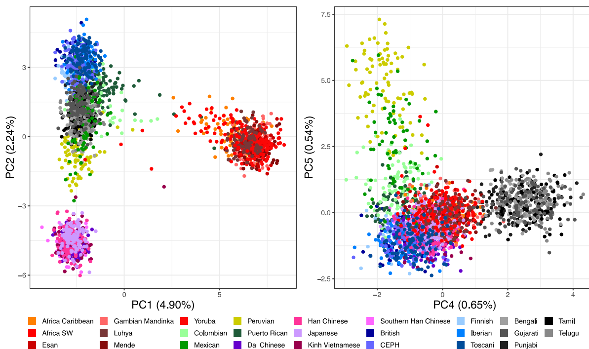
Figure 3. Principal Component Analysis (PCA) of common VNTR alleles in the NYGC population (150 bp). PCA was performed to reduce the dimensions of the data. Left: PC1 captured ~5% of the variation and separated Africans from the other super-populations, suggesting that they had the greatest distance from the others. PC2 separated East Asian and European populations but left individuals from the Americas and South Asia mixed. Right: PC4 separated the South Asian population and PC5 separated the American populations. PC3 (not shown) captured batch effects due to differences in coverage. Some American sub-populations proved hardest to separate, likely due to ancestry mixing.
