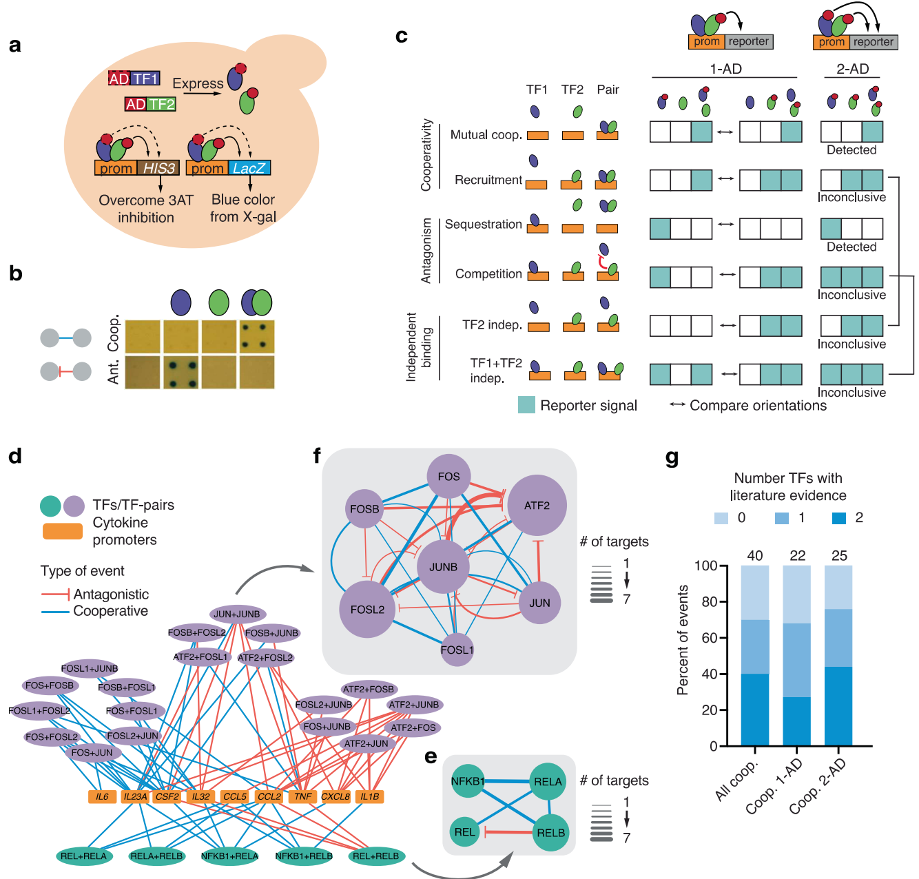
Fig. 1 | Paired yeast one-hybrid (pY1H) assays. a Schematic of pY1H assays. A DNA-bait yeast strain with a DNA sequence of interest (e.g., a promoter) cloned upstream of the HIS3 and lacZ reporter genes is mated with a TF-pair prey strain expressing two TFs fused or not to the Gal4 activation domain (AD). If an AD-containing TF binds the DNA region of interest, reporter expression will allow the yeast to grow in media lacking histidine and in the presence of the His3p inhibitor 3-amino-1,2,4-triazole (3AT), and turn blue in the presence of X-gal. b pY1H assays detect cooperative and antagonistic interactions by comparing single-TF and TF-pair yeast strains. c Comparison between 1-AD and 2-AD screen designs for different cooperative (mutual cooperativity and recruitment), antagonistic (sequestration and competition), and independent DNA binding modalities. Teal boxes indicate cases
